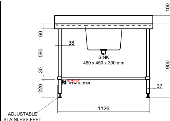
FRONT ELEVATION
